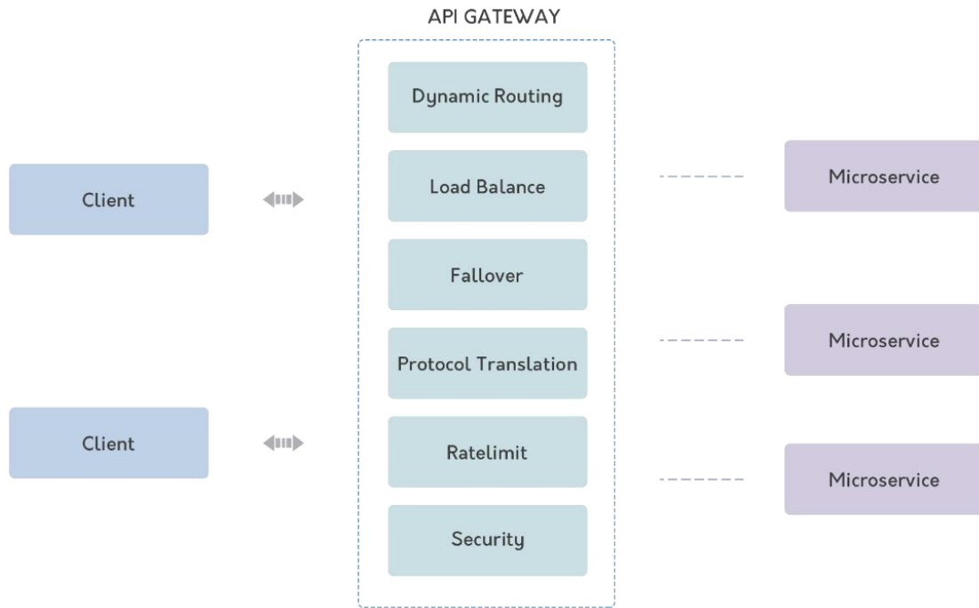
Figure 5.3.5.2 API Gateway
