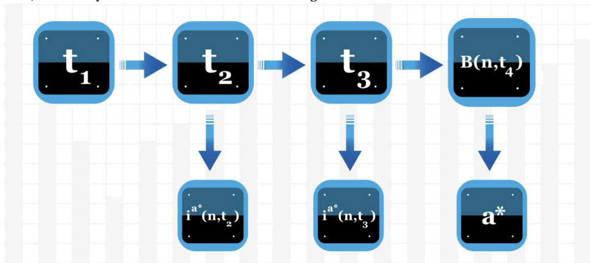
Figure 4.3.1 AM in PoA producing blocks
