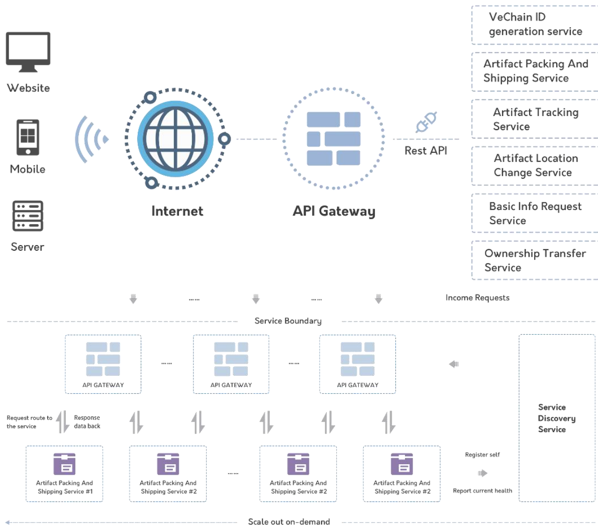
Figure 5.3.5.1 API Gateway-1
