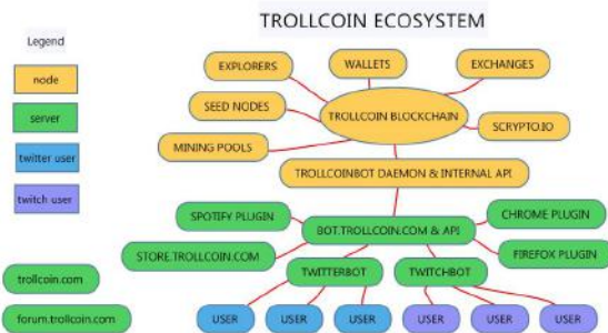
Figure 2. Trollcoin Ecosystem
