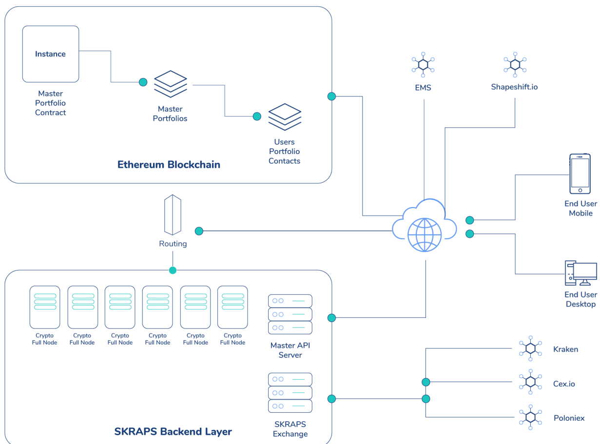
Fig 6. Skraps Technical Architecture
