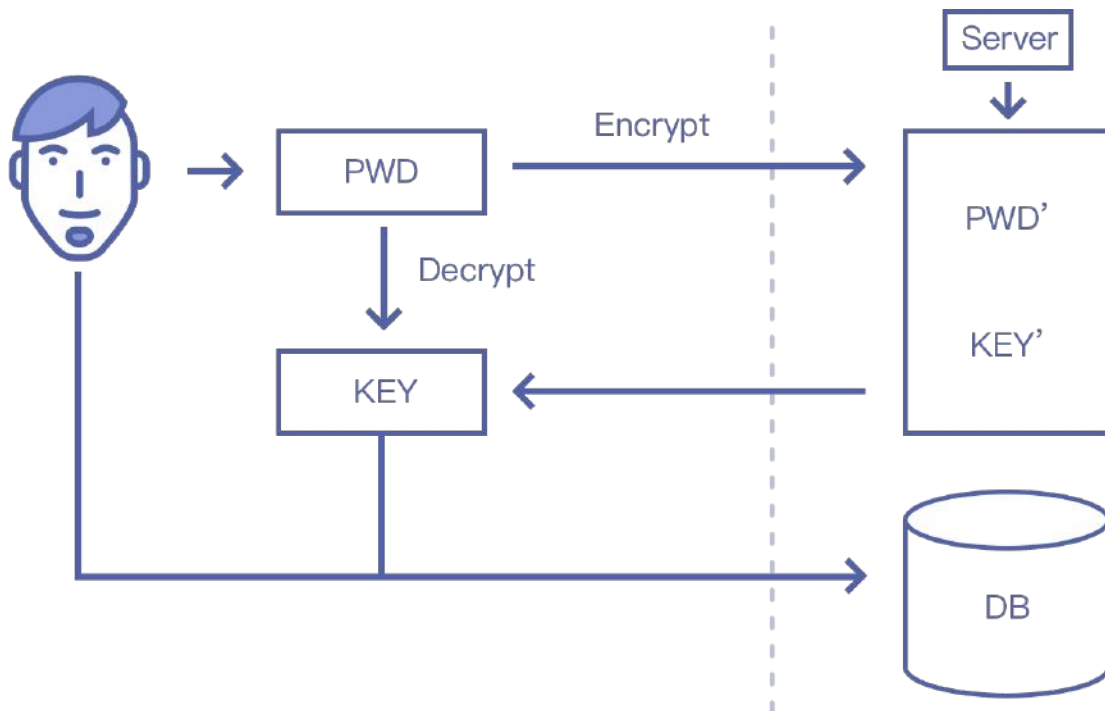
Figure 2 Retrieve the private key
