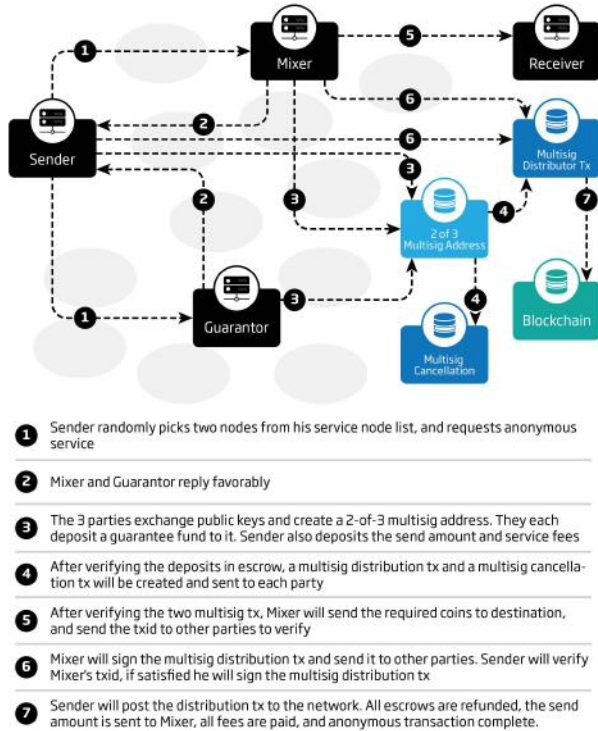
Fig. 3. DeepSend Transaction: Ofuscation through Coin-Join & Multi-signature
